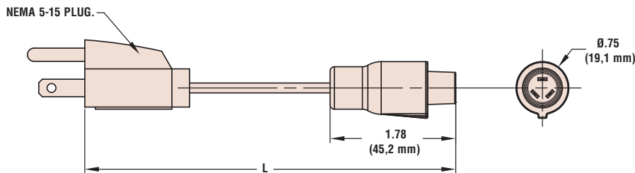
S7501-72 Power Cord
