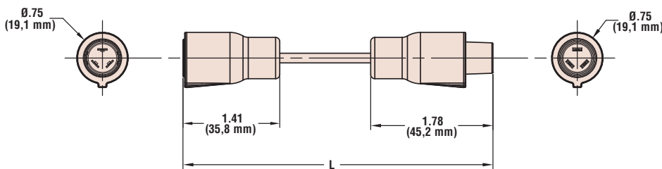
S7506 Jumper
