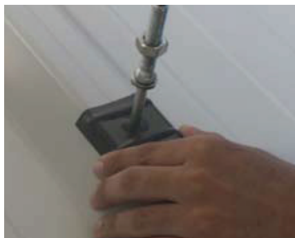
EJOT ORKAN Storm Washer for corrugated metal profiles
