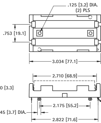
Mounting Detail
