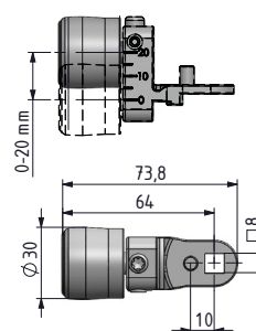
Adjustable cam (Round roller)
