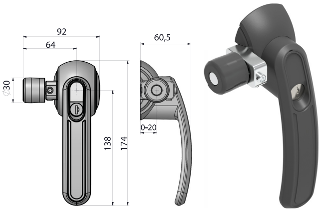
Handle for inward opening doors
