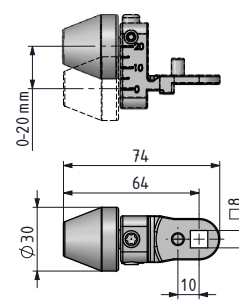
Adjustable cam (Triangle Roller)
