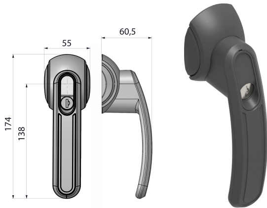
Handle for outward opening doors
