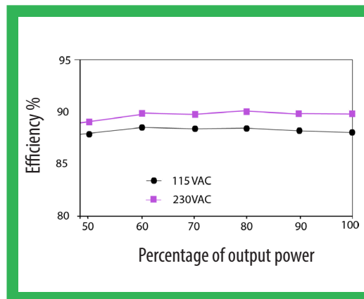
Figure 1: The efficiency of a supply varies with load, and most peak in the zone of 80-95% of their maximum rated capacity; this chart shows the N2Power XL280 curve.
